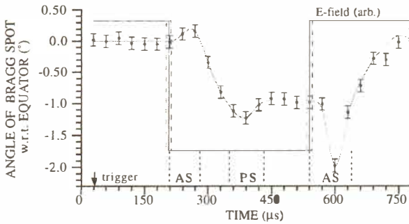
FIGURE 5 The angle of the Bragg spot relative to the equator, as a function of time. Each data point represents the accumulated intensity in the preceeding 30 \mu s.
